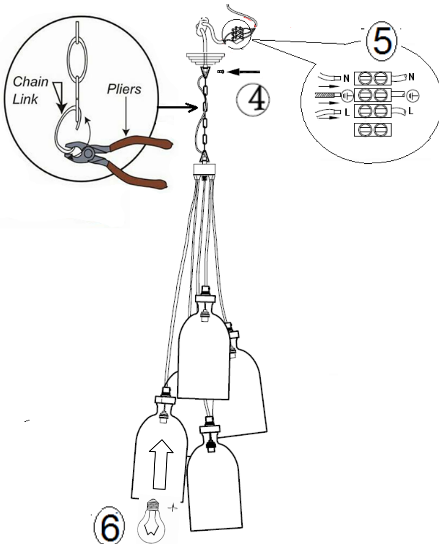
Wiring Details
