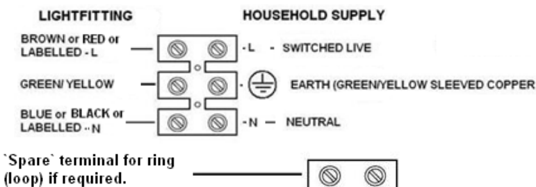
Wiring Details
